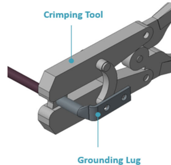
Crimping tool
