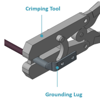
Crimping tool
